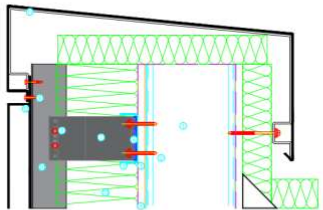
Spanwall SF40-FR Rainscreen Parapet Coping
